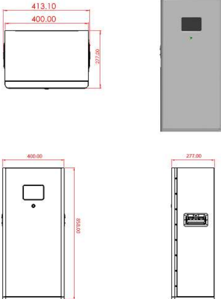
Battery module size diagram
