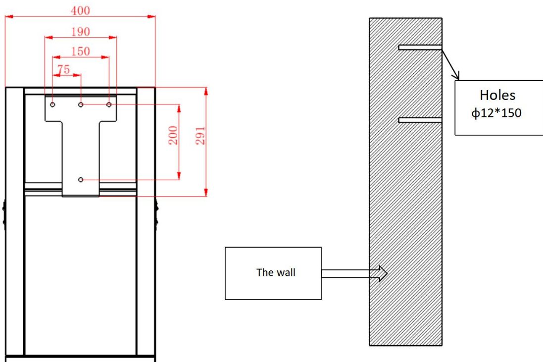
Mounting bracket size drawing
