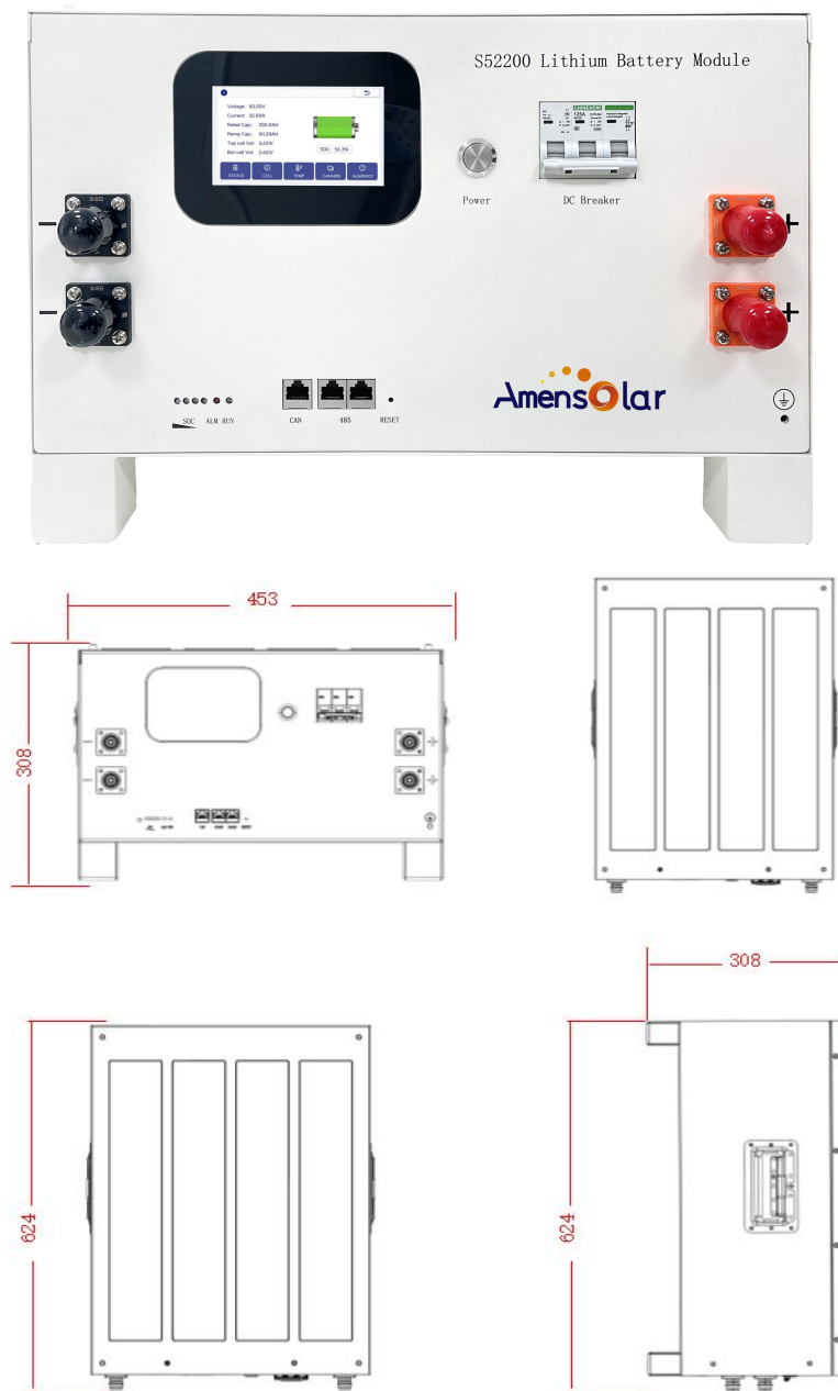
Battery module size diagram
